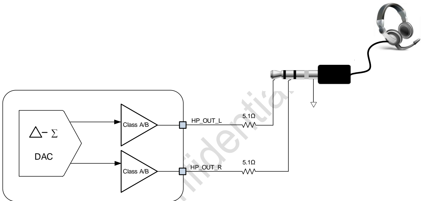
Figure 3. Output signal path diagram
