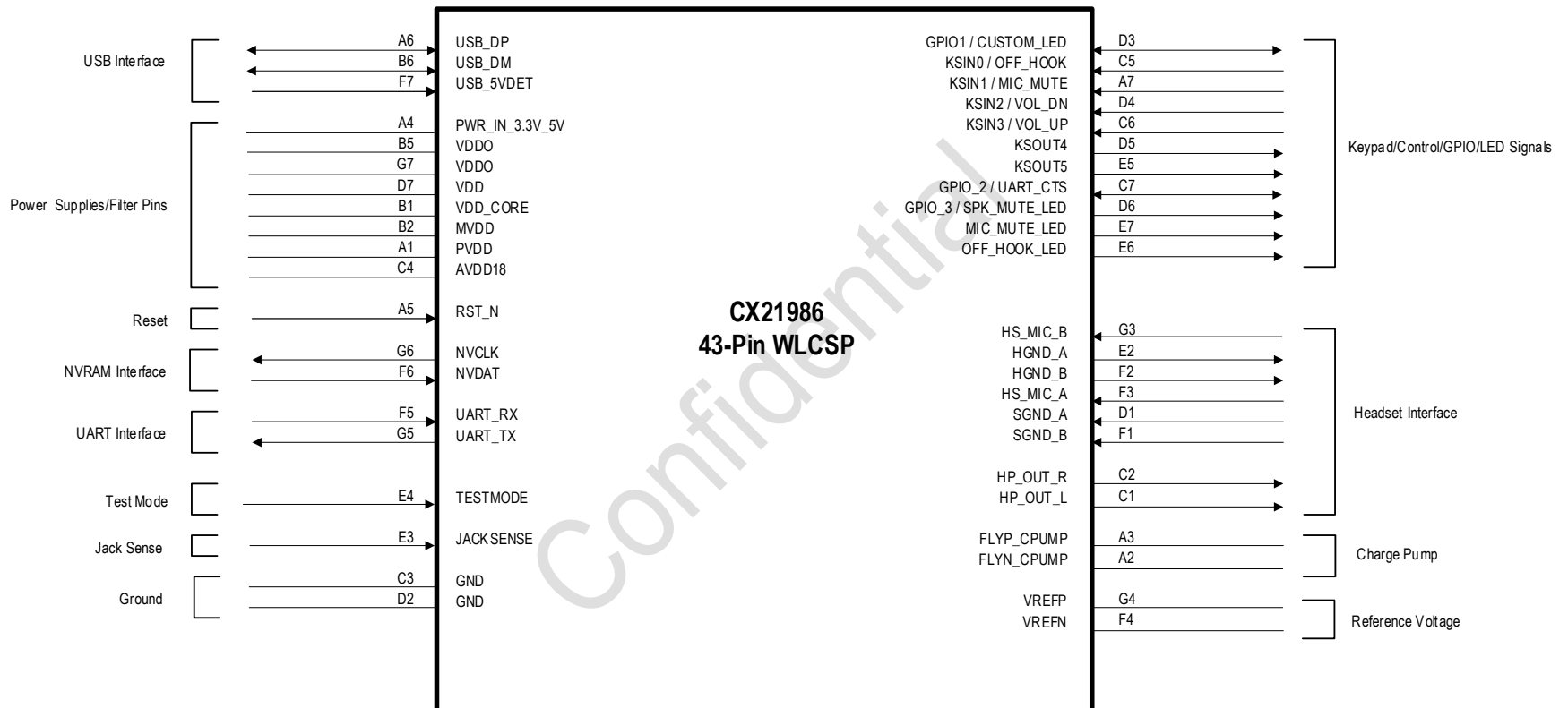
Figure 17. CX21986 43-pin WLCSP hardware interface signals
