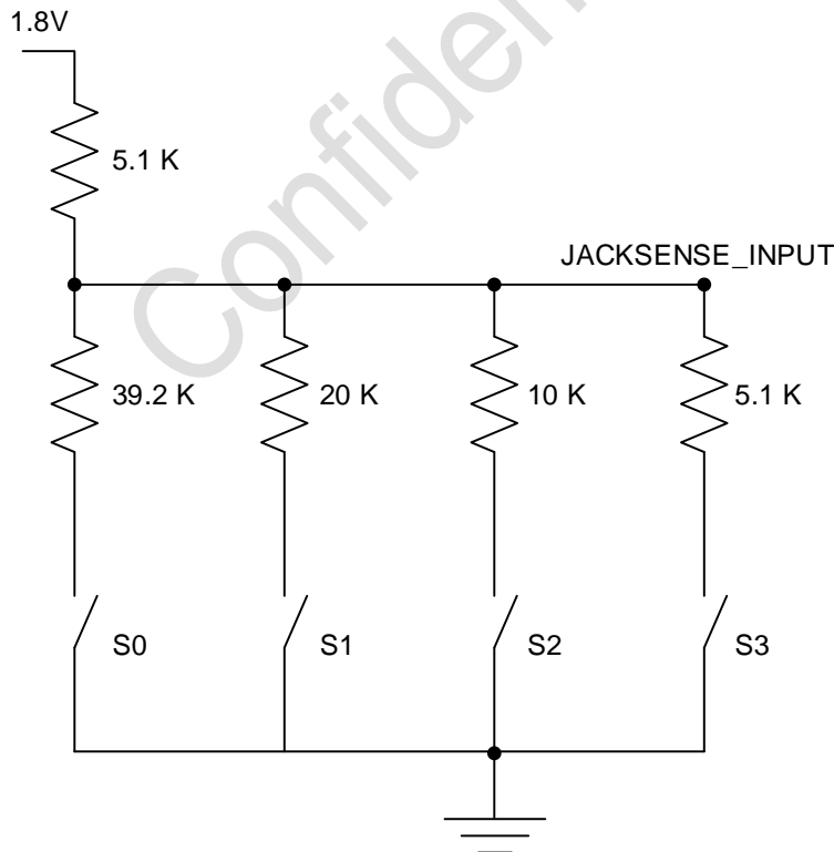
Figure 8. External circuit
