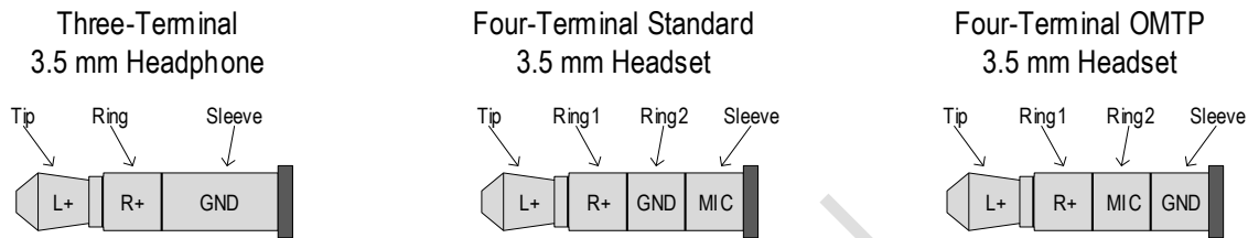
Figure 6. Multi-standard headset support
