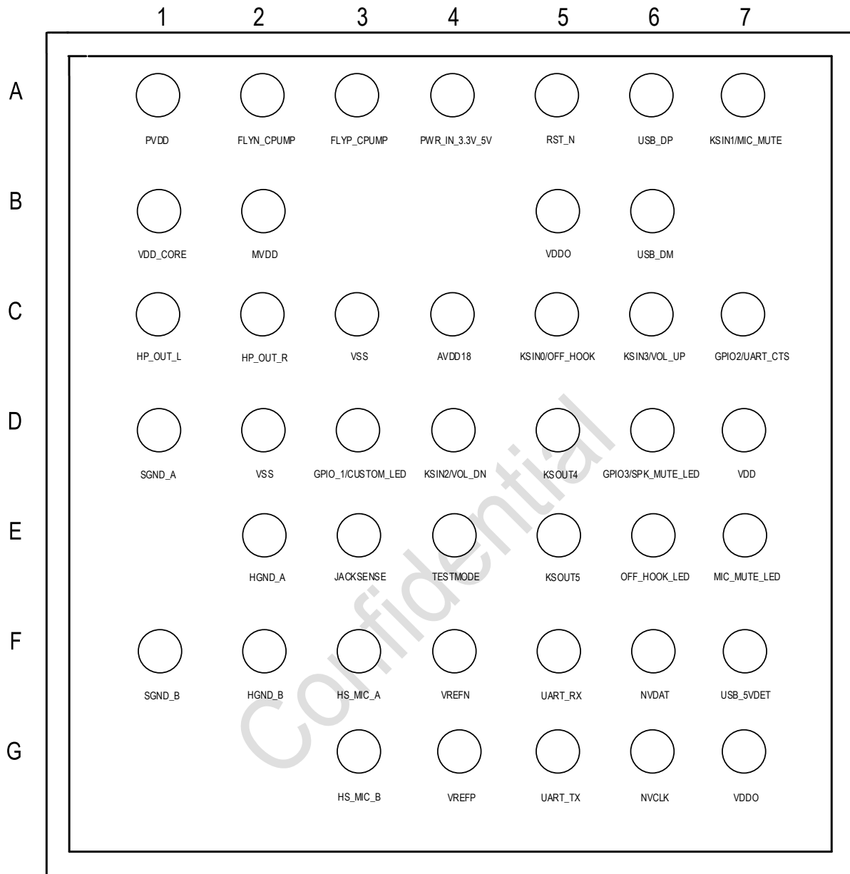
Figure 18. CX21986 43-pin WLCSP pin signals
