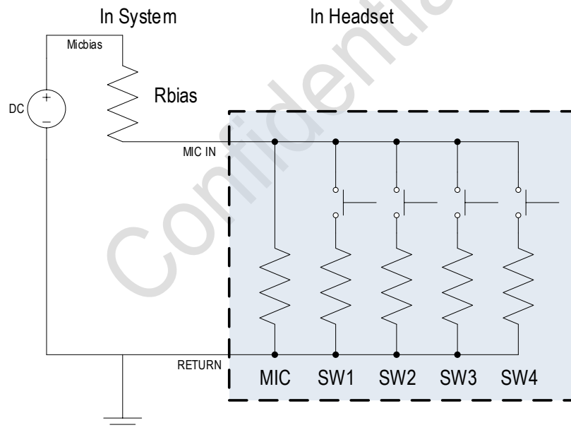
Figure 9. Microphone button detect
