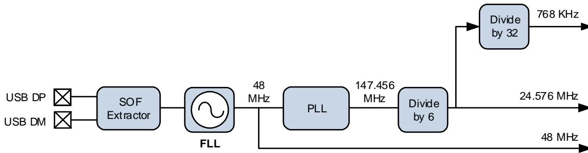
Figure 13. On-chip reference clock generation
