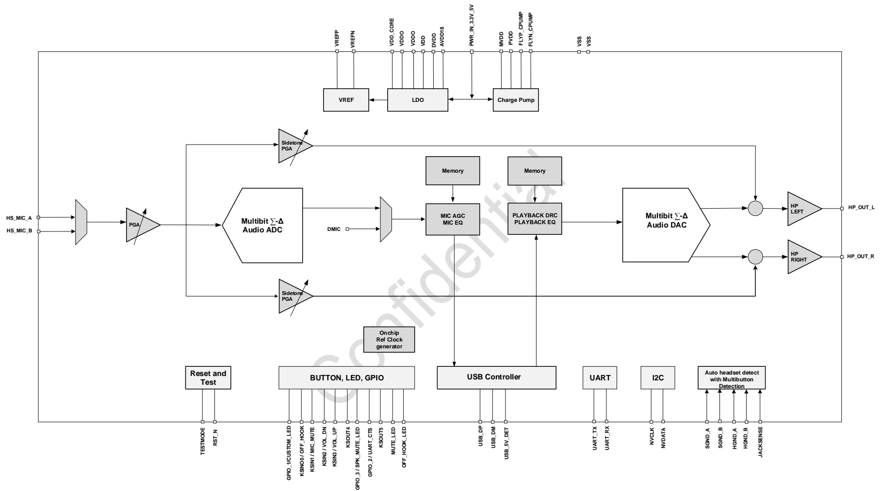
Figure 1. CX21986 system block diagram
