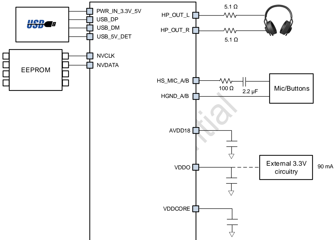
Figure 16. USB Type-C headset with android button support block diagram
