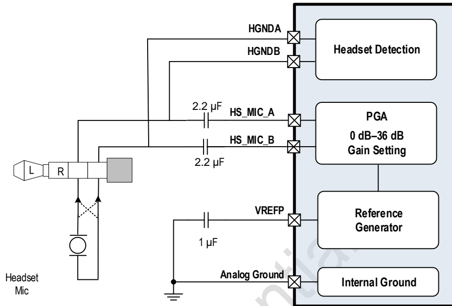
Figure 2. Headset micbiasing configuration
