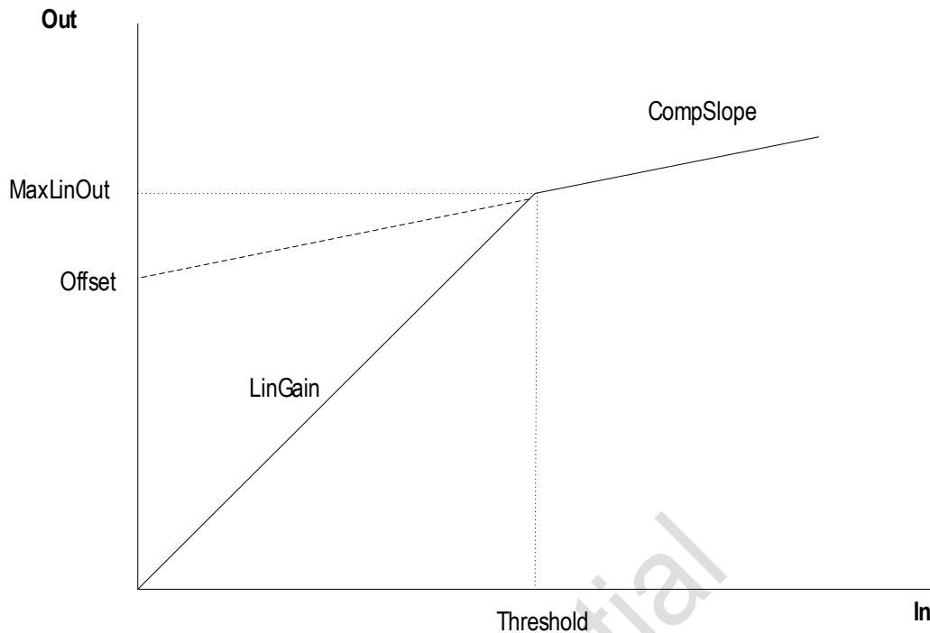
Figure 5. DRC curve
