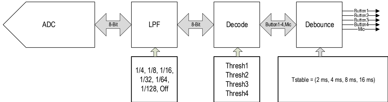
Figure 10. ADC clocked at 768 kHz
