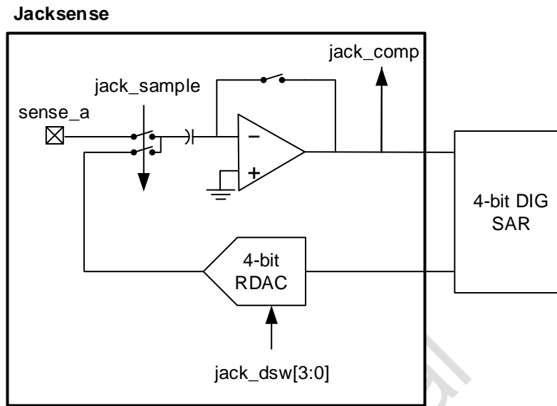
Figure 7. Jack sensing
