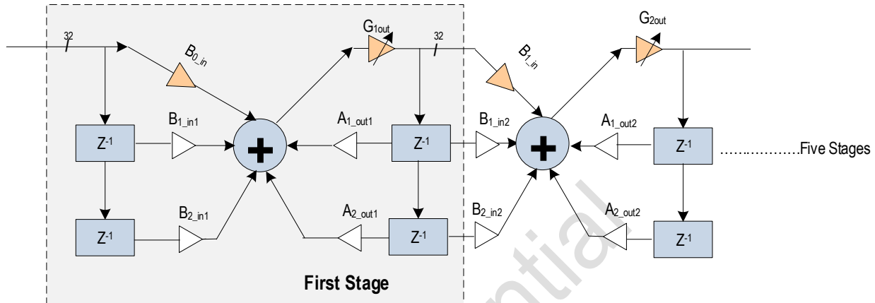
Figure 4. EQ block diagram
