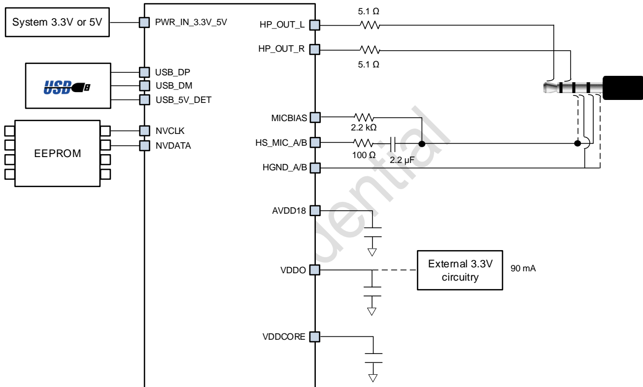
Figure 15. USB Type-C audio adapter docking station and audio adapter block diagram
